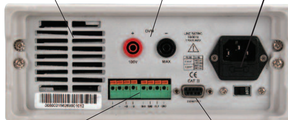
Serial interface connector for RS232 or USB communication. (USB communication cable is optional). Model 9123A also supports control via GPIB interface.
